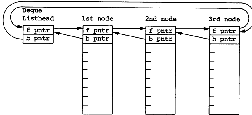
Figure 1-1 A Three-Node Deque
